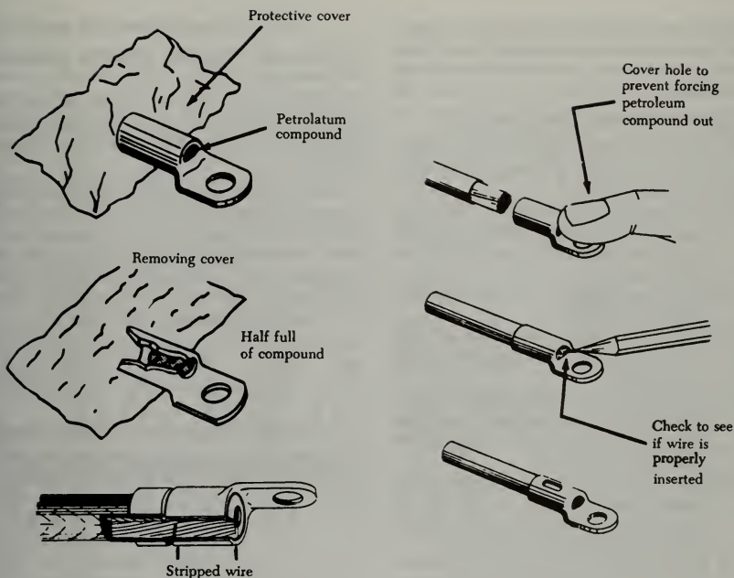
FIGURE 4-109. Inserting aluminum wire into aluminum terminal lugs.
